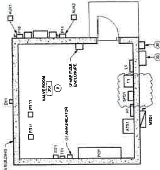
1 LIFT STATION BUILDING CONTROL PLAN 1/4" = 1'-0"
